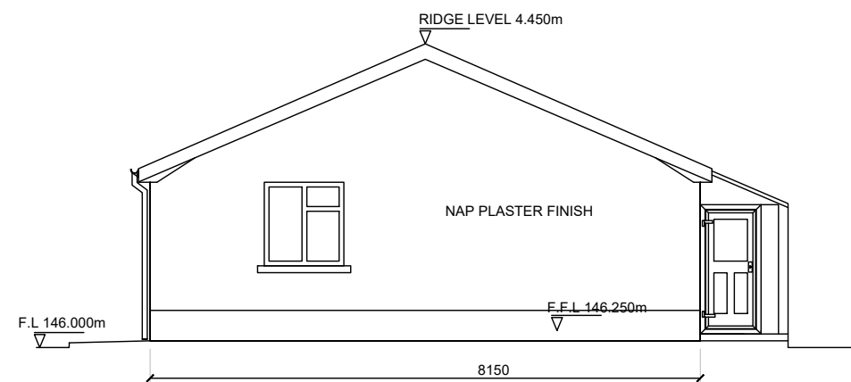
SIDE ELEVATION - WEST FACING SCALE; 1:100
